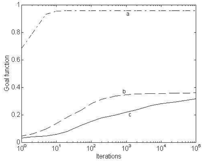
Figure 3. EA with both types of operators: a - N=10 , b - N=100 , c - N=1000
