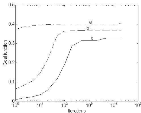
Figure 7. EA with both types of operators: a - N=10 , b - N=100 , c - N=1000
