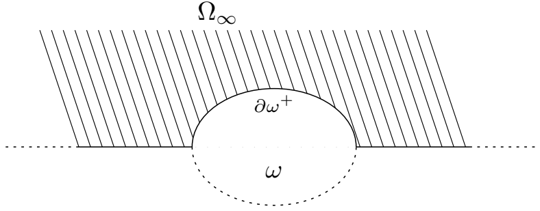
Figure 2. The limit domain
