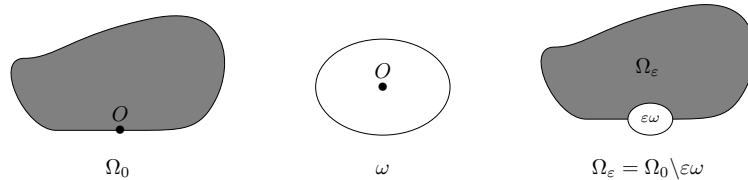
Figure 1. The geometrical setting
