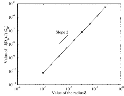
Figure 4. Comparison between J(\Omega_\varepsilon) and J(\Omega_0) with respect to \varepsilon (logarithmic axes)
