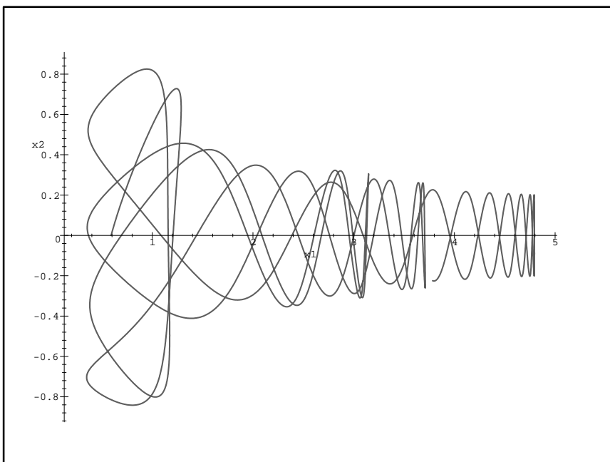
Fig. 8. Typical trajectory of the system with Hamiltonian (16)
