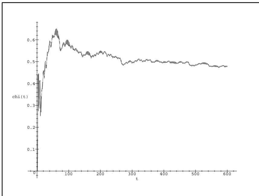
Fig. 6. The example of the Lyapunov exponent for the two-dimensional system, obtained in the su(3) case
