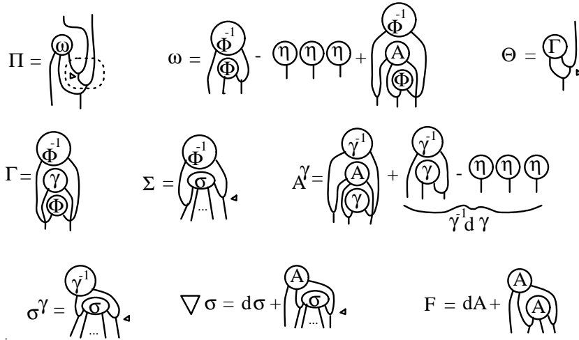
Figure 3: Braided gauge theory of ‘enveloping algebra’ type
