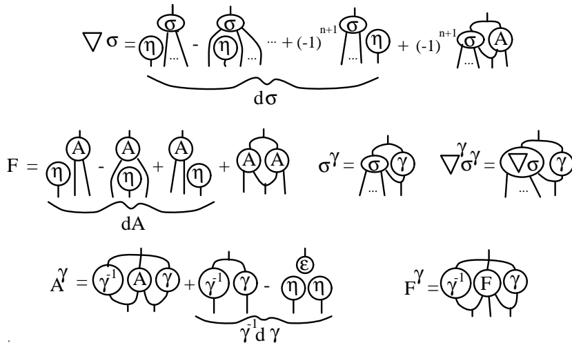
Figure 2: Local form of braided gauge theory
