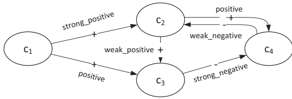
Fig. 1. Example of an FCM graph. Vertices are assigned with concepts, directed arcs with linguistic weights of specifying influence.
