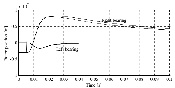
Fig. 16. Rotor positions—the global model (simulation).
