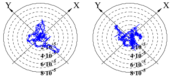
Fig. 20. Trajectory of the rotor position in left and right bearings.
