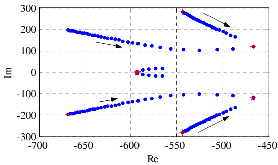
Fig. 22. Root location for the closed-loop system with the LQ controller designed for \Omega = 30\ 000 1/s and decreased to 0.
