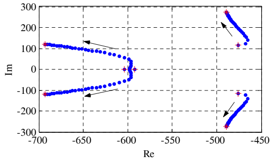
Fig. 21. Root location for the closed-loop system with the LQ controller designed for \Omega = 0 and increased to 30 000 1/s (simulation).
