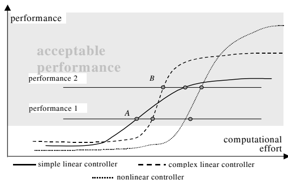
Fig. 1. Control performance and computational effort.
