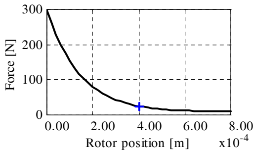
Fig. 11. Force vs. the rotor position for a fixed value of the current.
