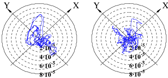
Fig. 18. Trajectory of the rotor position in left and right bearings.
