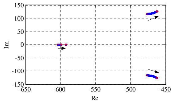
Fig. 23. Root location for the closed-loop system with LQ controller parameters adapted for each rotational velocity, \Omega \in [30000, 0] .
