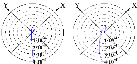
Fig. 5. Loading the rotor, the distance between the rotor axis and the bearing centre [m].
