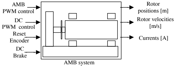
Fig. 4. MATLAB/Simulink interface.
