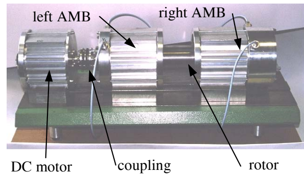
Fig. 3. Active magnetic bearing, laboratory model.
