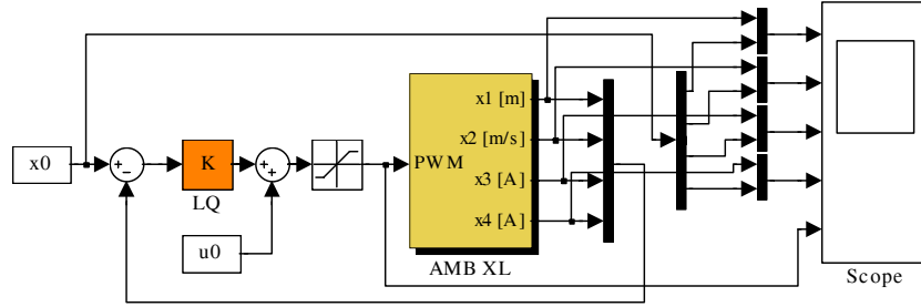
Fig. 13. MATLAB/Simulink local LQ controller loop for a single axis.
