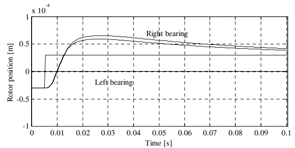
Fig. 15. Rotor positions—the local model (simulation).
