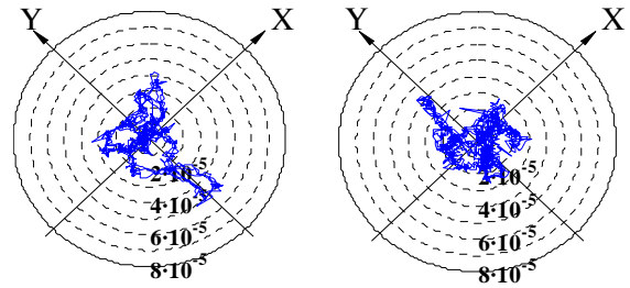
Fig. 19. Trajectory of the rotor position in left and right bearings.
