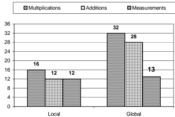
Fig. 24. Computational effort: comparison of local and global controllers.
