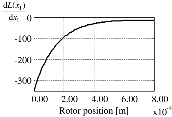
Fig. 9. Coil inductance vs. the rotor position.
