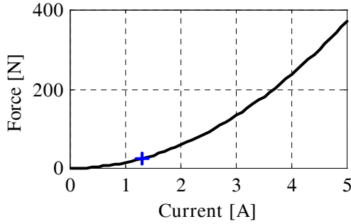
Fig. 10. Force vs. current for a fixed rotor position.
