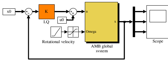
Fig. 14. MATLAB/Simulink global LQ controller loop.
