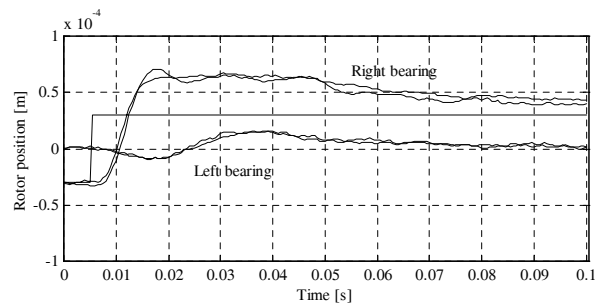
Fig. 17. Rotor positions—an experiment (the global model).
