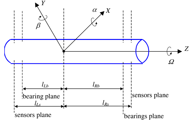
Fig. 12. Full model of the rotor.
