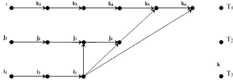
Fig. 2. Monomial tree.
