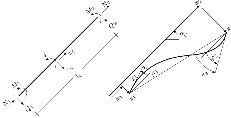
Fig. 21. Released prismatic member.
