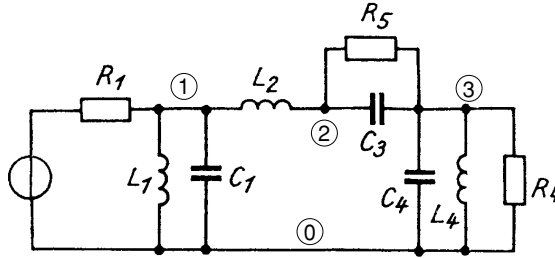
Fig. 10. Example of an RLC-network.
