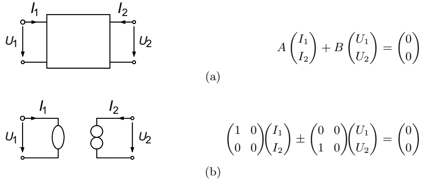
Fig. 8. Two-port network elements: (a) general two-port and its NERs, (b) nullor and its NERs.
