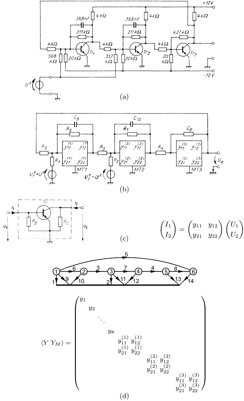
Fig. 11. Active RC circuit: (a) RC circuit with three transistors, (b) small signal network model, (c) admittance representation of a transistor, (d) network graph and branch admittance matrix.
