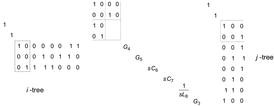
Fig. 15. Network determinant for the example of Fig. 13.
