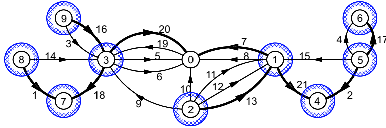
Fig. 4. Independent node cut sets and one possible set of tree branches.
