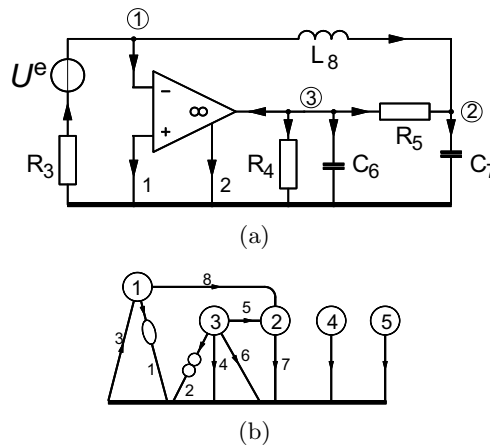
Fig. 13. Network model and augmented network graph.
