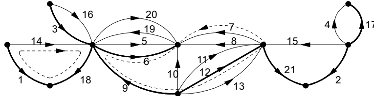
Fig. 5. A spanning tree in the network graph and the two basic meshes that are defined by the links 7 and 14.
