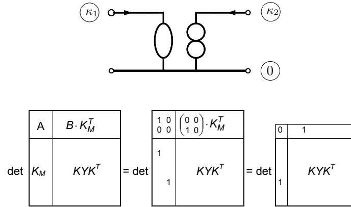
Fig. 17. The determinant of a network augmented by an added nullor as indicated is equal to the (\kappa_1, \kappa_2) -cofactor of the original network determinant.
