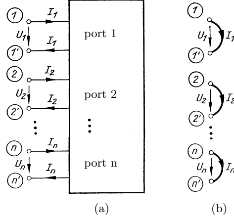
Fig. 7. General n -port: (a) pictorial representation of an n -port network element, (b) representation as part of the network graph.
