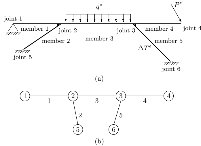
Fig. 20. Plane framework and its corresponding graph.
