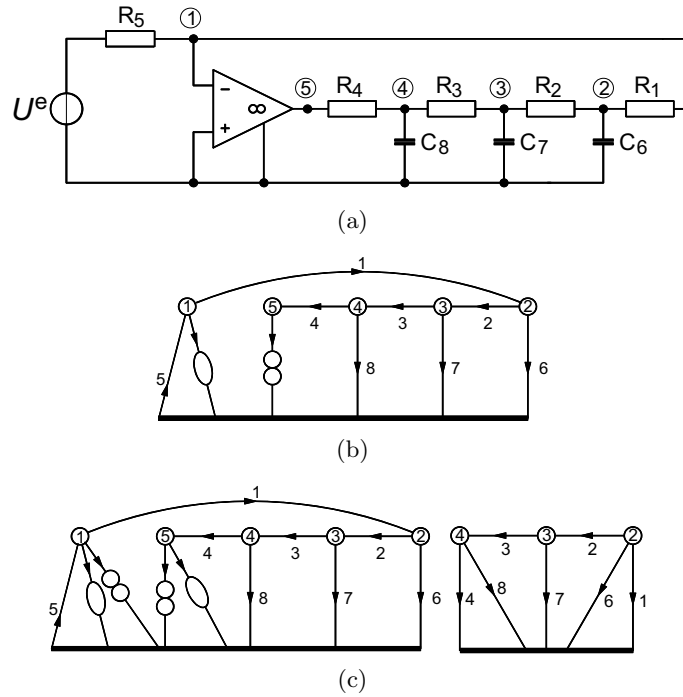
Fig. 18. (a) RC network with one operational amplifier, (b) network graph for the network determinant, (c) network graphs for the numerator polynomial.
