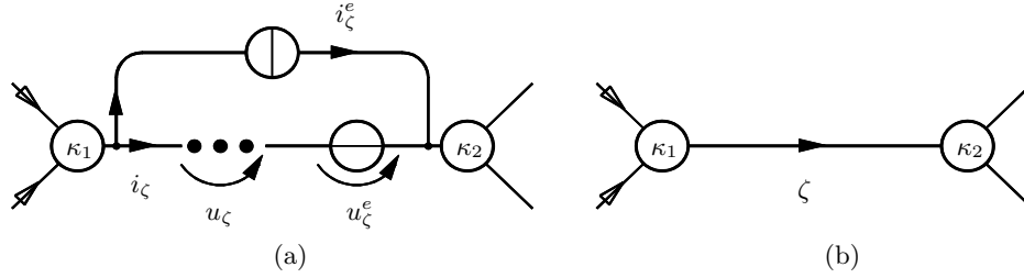
Fig. 6. General form of a branch: (a) pictorial representation of branch \zeta leading from node \kappa_1 to node \kappa_2 , (b) branch \zeta as part of the network graph.
