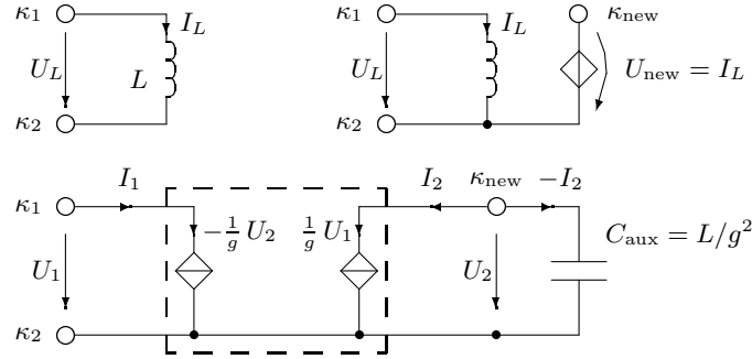
Fig. 12. Two possibilities to get modified nodal equations whose coefficients are affine functions of the complex frequency s .
