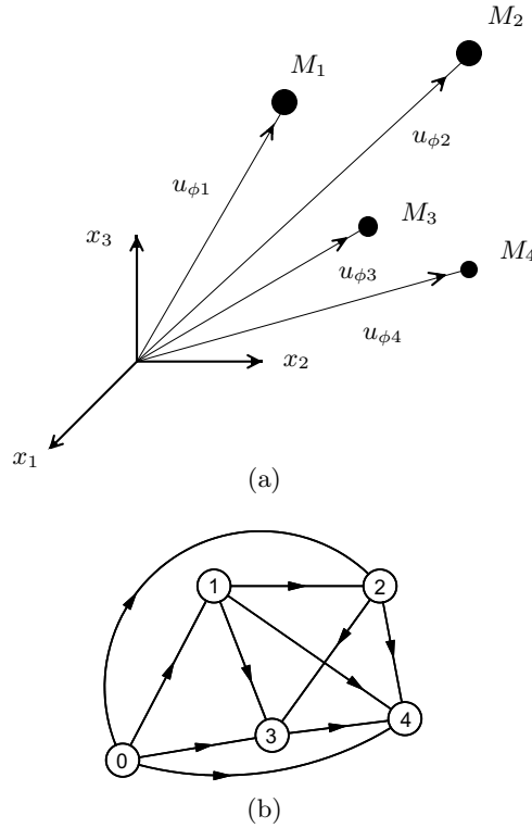
Fig. 19. Newtonian n -body problem: (a) pictorial representation for n = 4 , (b) network graph for n = 4 .
