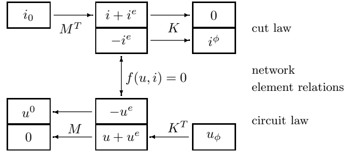
Fig. 9. The three ingredients of network models.
