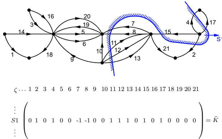
Fig. 2. Oriented cut-set and cut-set branch incidence matrix.
